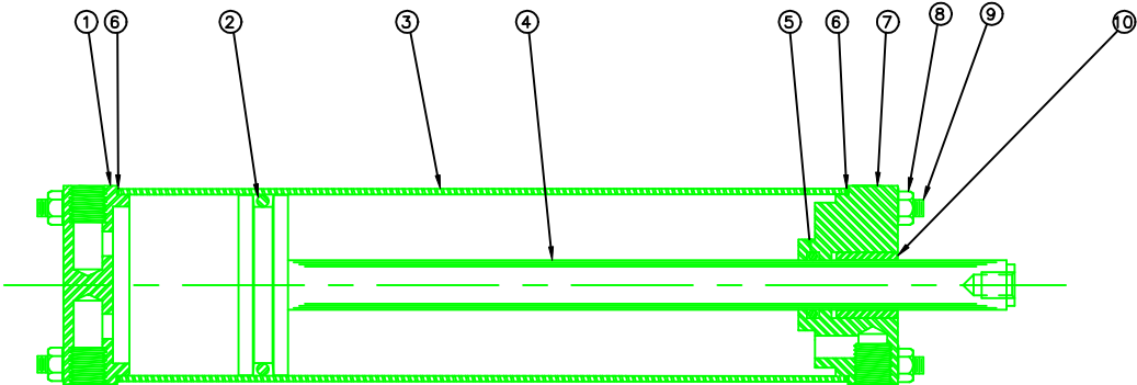
FRONT HEAD CLOSING CYLINDER #A-3759
