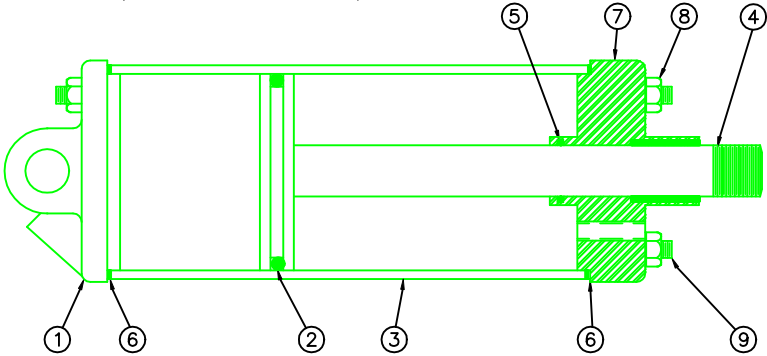
BUCK TRANSFER CYLINDER (Part No. A-5130)
