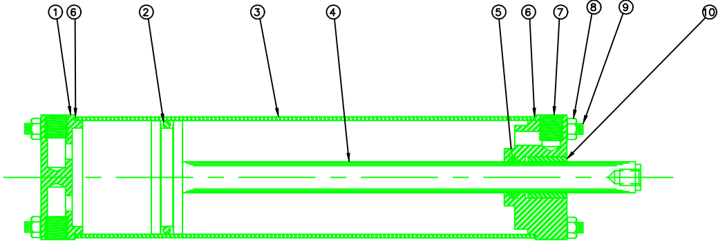
REAR HEAD CLOSING CYLINDER #A-3753
